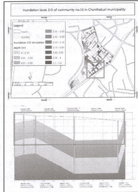
Figure 7 Inundation level 2-D of community no. 15 in Chanthaburi Municipality
